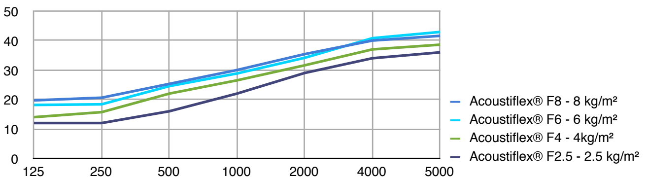
Field Transmission Loss (dB) for Acoustiflex® F
